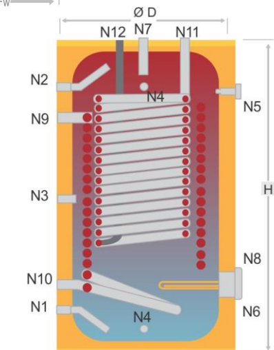
KXD DOUBLE SERPANTINE WATER HEATER ( 200 lt - 300 lt - 500 lt )
