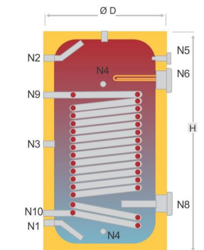
KXS SINGLE SERPANTINE WATER HEATER ( 1000 lt - 2000 lt )
