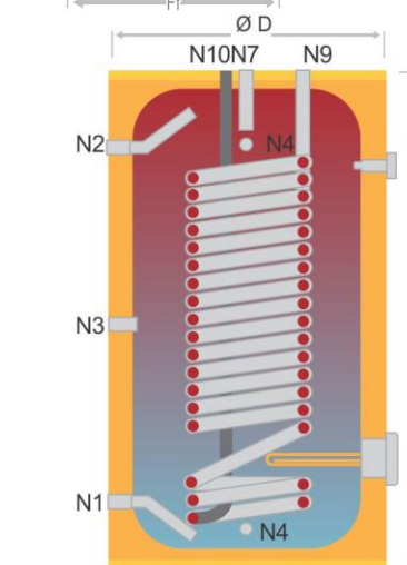
KXS SINGLE SERPANTINE WATER HEATER ( 100 lt - 200 lt - 300 lt - 500 lt )
